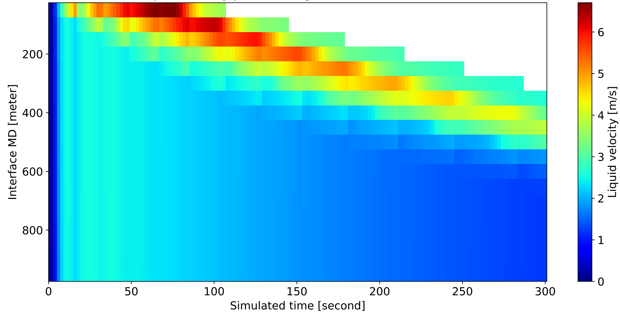
Liquid velocity profile along the wellbore over time
